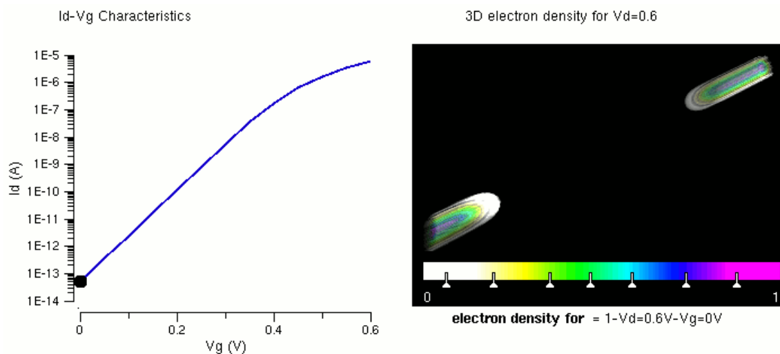
Fig. 13: One of the major applications of the nanotechnology is in the era of nanoelectronics with MOSFET 's is being made of small nanowires \sim 10\text{nm} in length. Here is a simulation of such a nanowire.
